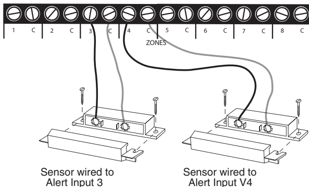
Figure 2-7. Two Sensors Wired to Adjacent Zones
