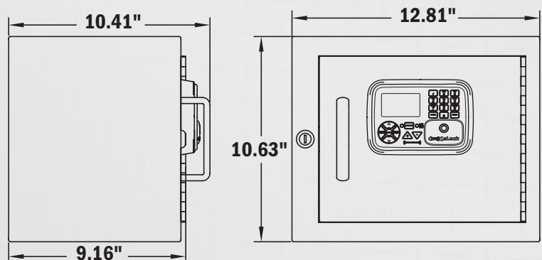
Narcotics box dimensions with CompX eLock installed
